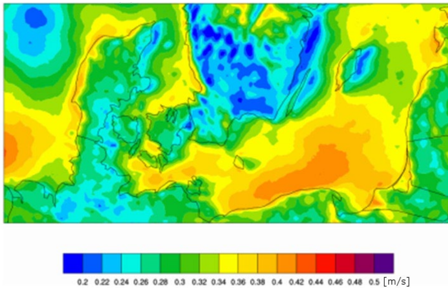
Fig. 7. Standard deviation ( \text{ms}^{-1} ) in the mean annual wind speed at the height of 100 m – average for a specific period (2006–2011) Source: Hahmann et al. 2012
