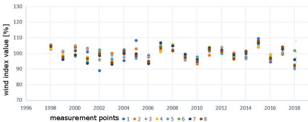
Fig. 3. Values of wind indexes over the last twenty years Source: own study based on (Solar Energy Services for Professionals 2018)
