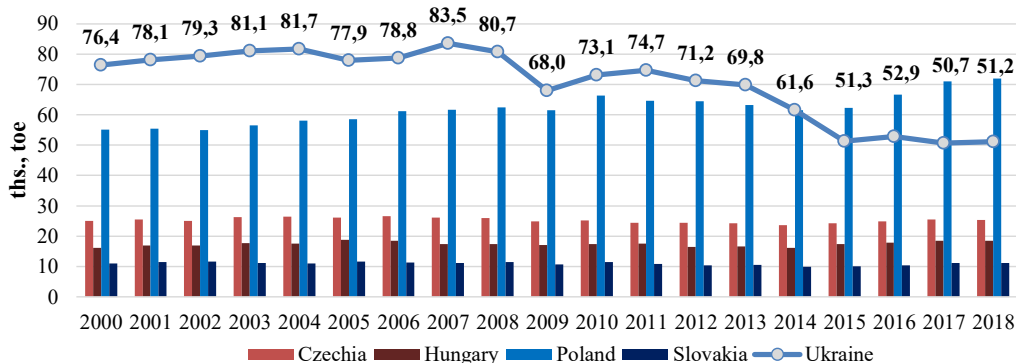
Fig. 2. Final energy consumption of Ukraine and V4, 2000–2018 Source: compiled by the authors based on data from (Eurostat 2020)
