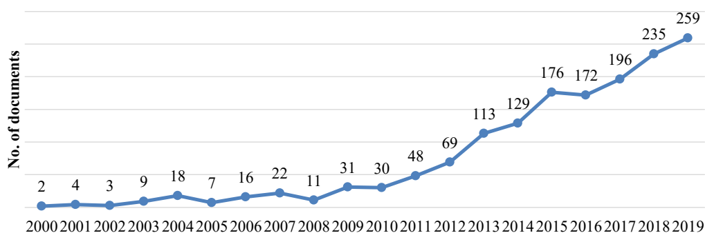
Fig. 4. The dynamic of publication activity on energy-efficient gaps, 2000–2019 Source: developed by the authors based on (Scopus 2020)
