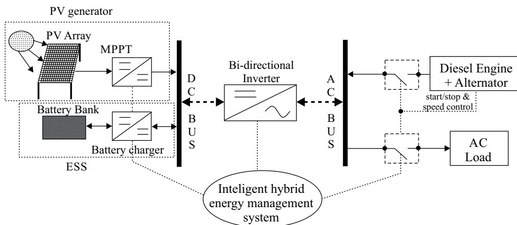
Fig. 2. Parallel PV–diesel–battery system
