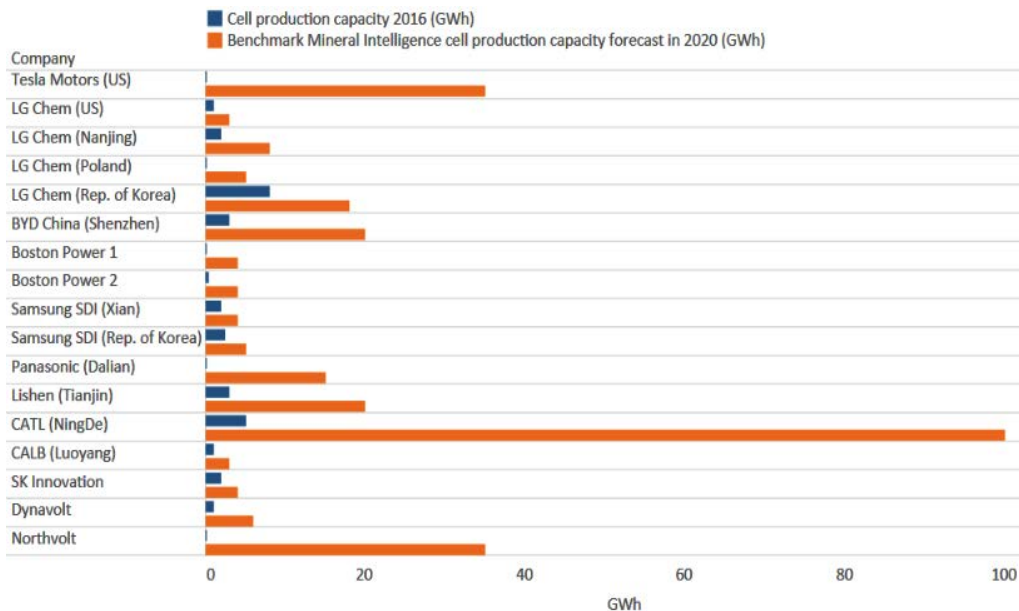
Fig. 10. Production capacity forecast for producers of lithium-ion batteries Source: IRENA 2017
