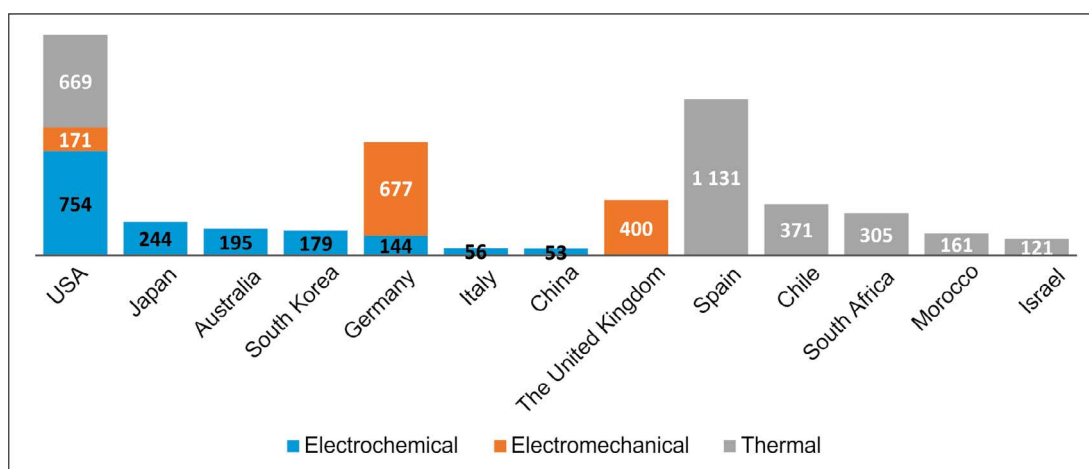
Fig. 1. The installed capacity of energy storage (non-PSH) at the end of 2017 [MW] Source: U.S. DOE 2018
