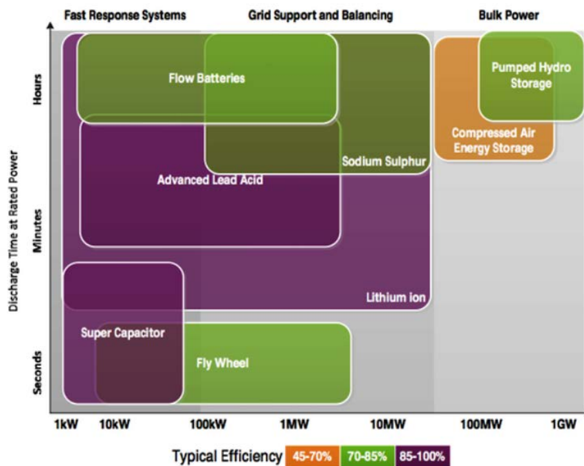
Fig. 5. Storage technologies from the point of view of efficiency, capacity, response time, and discharge time Source: CleanTechnica 2015
